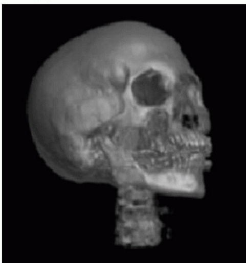
Shear-Warp
